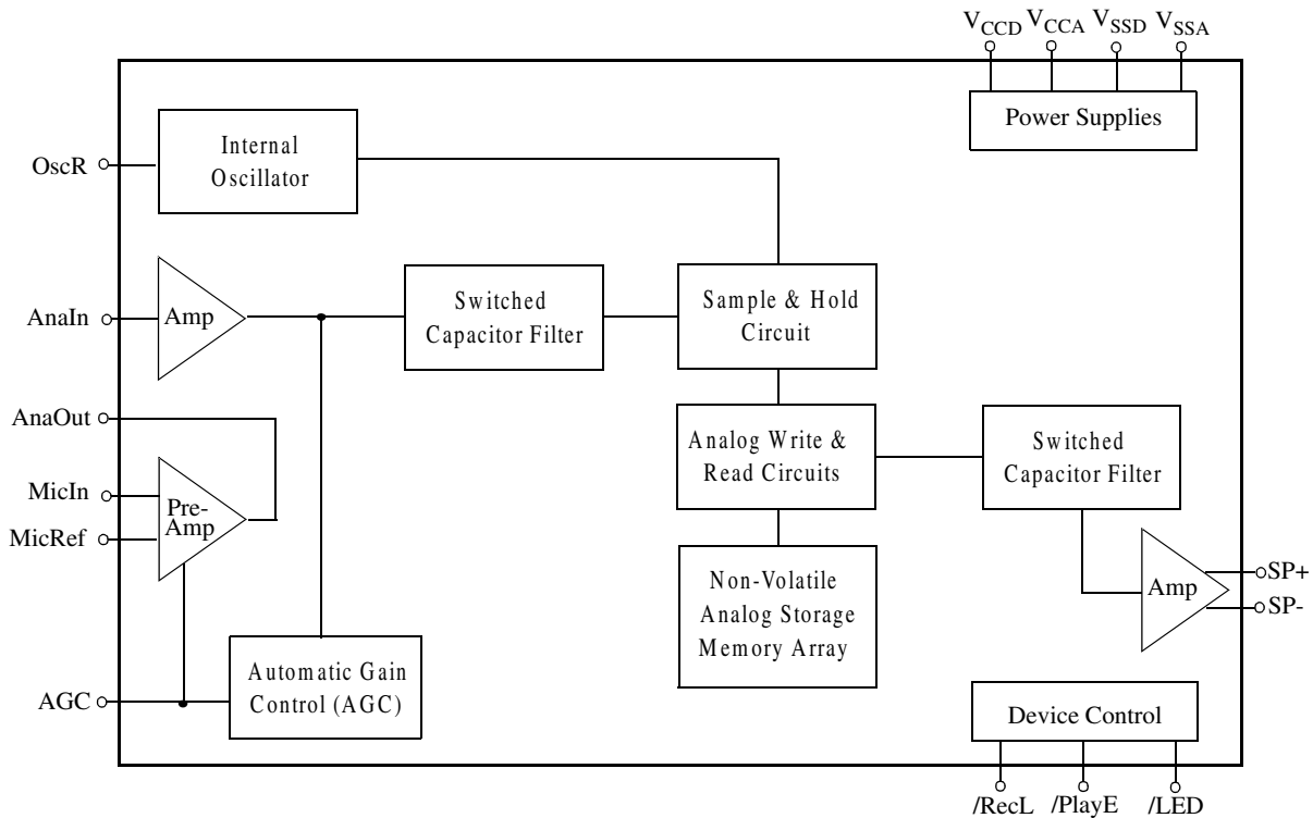
Figure 2 AR9301 -V2 Functional Block Diagram
